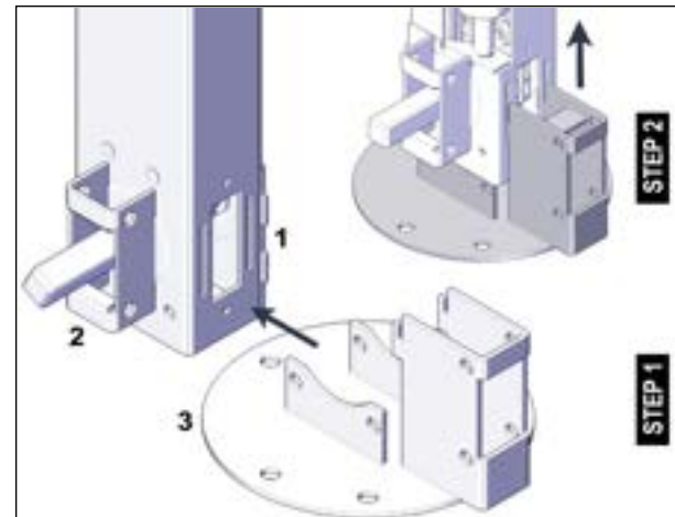
FIGURE 8: INSTALL FOOT BRACKET
