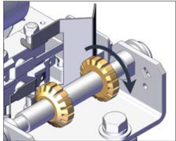
FIGURE 74: TURN UP-CAM WHEEL
