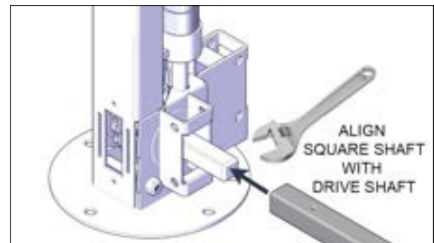
FIGURE 11: SLIDE DRIVE SHAFT OVER SQUARE SHAFT
